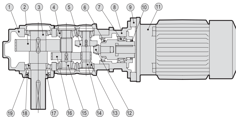
Drive Unit Right Angle Shaft Triple Reduction
