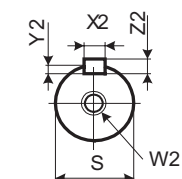
High Speed Shaft
